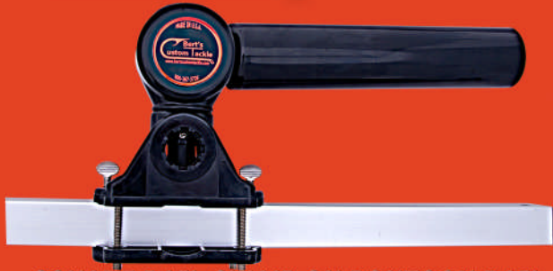
SQUARE RAIL CLAMP ON PONTOON RAIL
